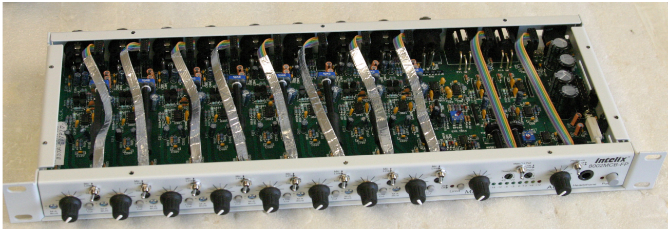
Internal picture of the 8002MCB-FP after the retrofit. Notice the 8 shielded ribbons (left-most) and the two unshielded ribbons (right-most).
