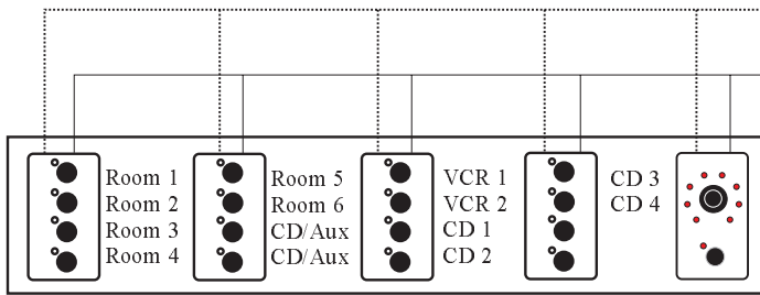
Room Combine and Program Select Stations (same for Rooms 1-6)
